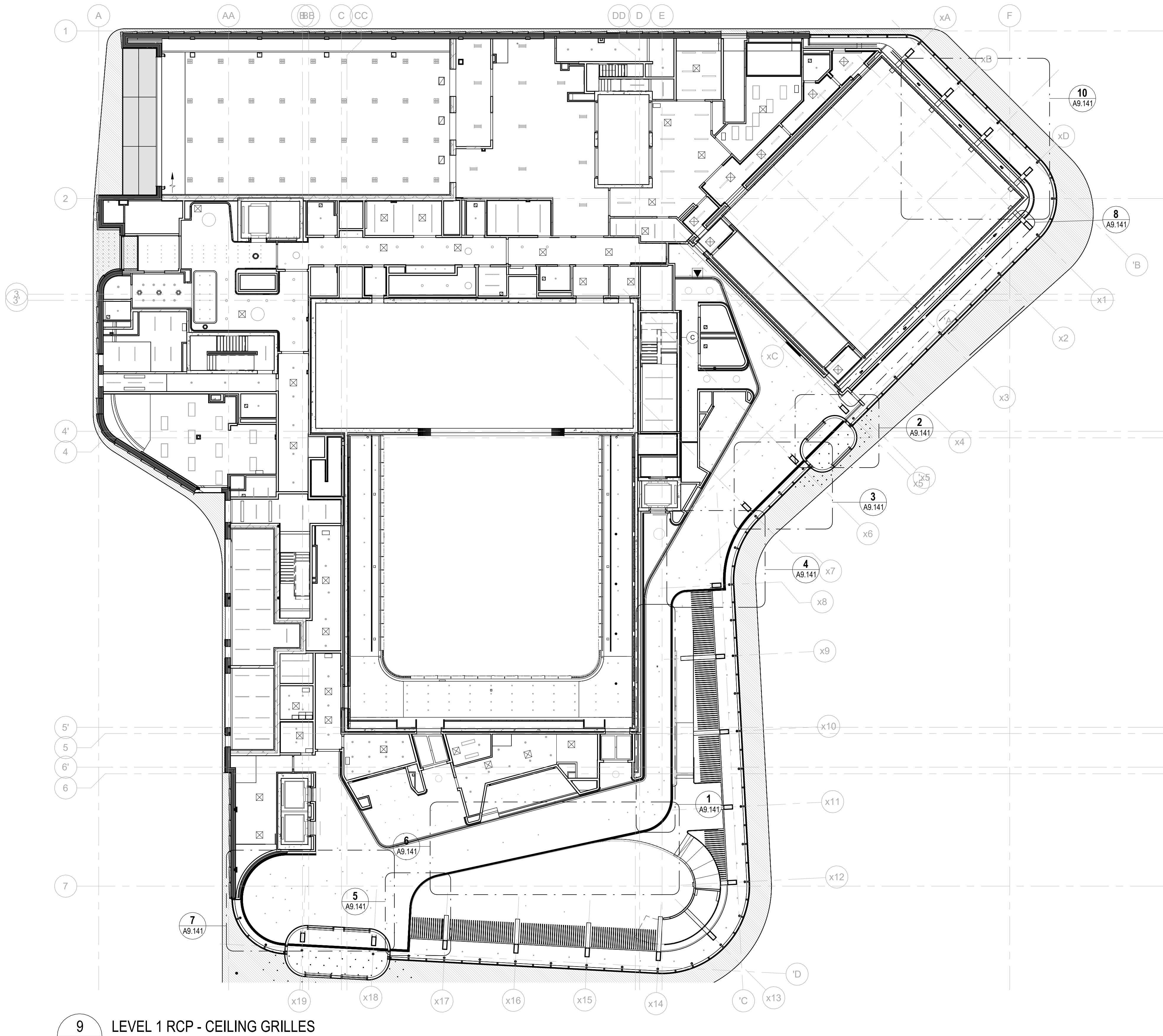
10 LEVEL 1 RCP - CEILING GRILLES - 9
