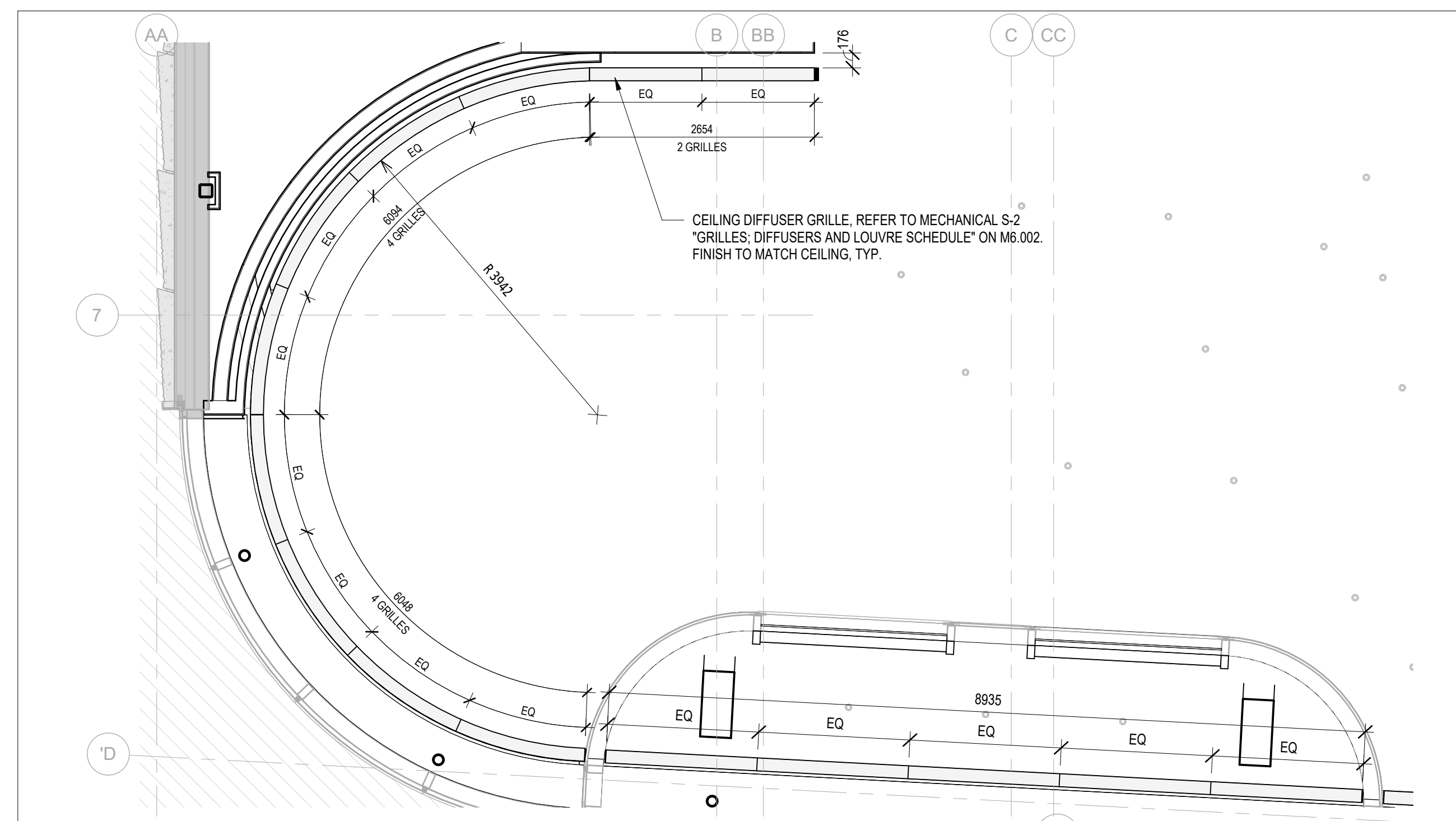
7 LEVEL 1 RCP - CEILING GRILLES - 7
