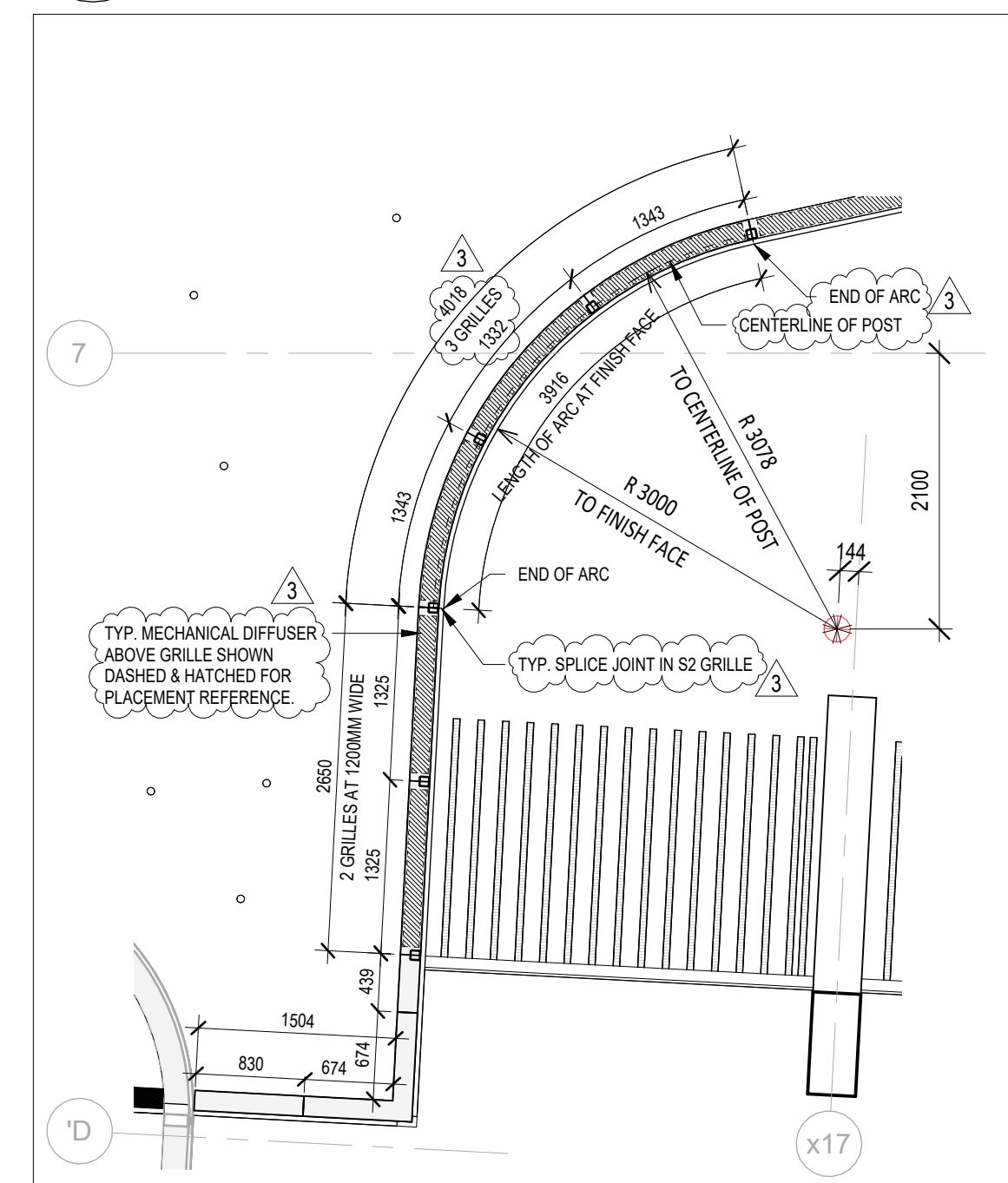
5 LEVEL 1 RCP - CEILING GRILLES - 4
