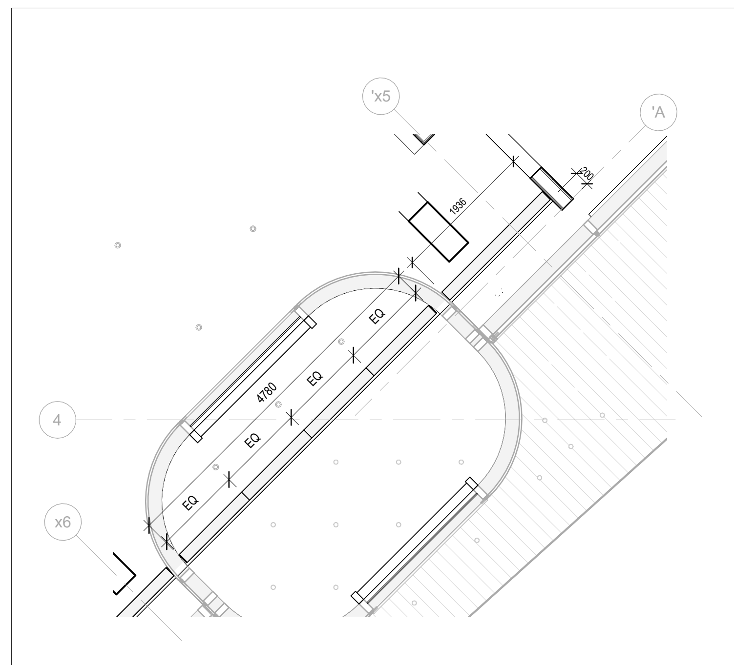
2 LEVEL 1 RCP - CEILING GRILLES - 1
