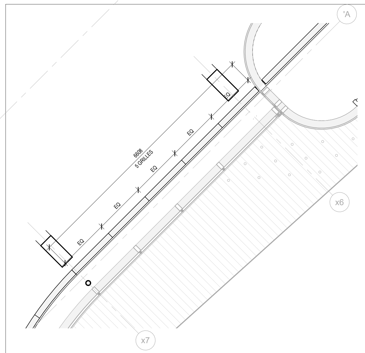
3 LEVEL 1 RCP - CEILING GRILLES - 2
